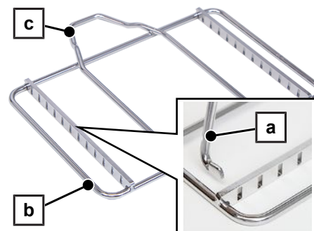
Insert the bracket into the base
