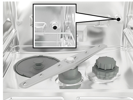
Inserting the basis basket
