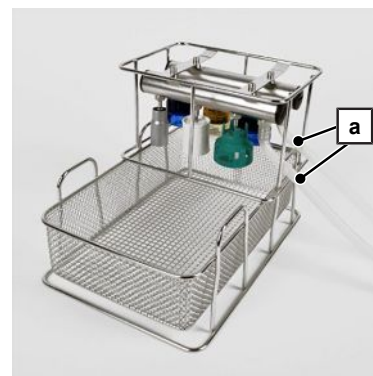
Flex basket 2 with injector basket Flex 1
