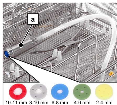
Connection example, rinse sleeve
